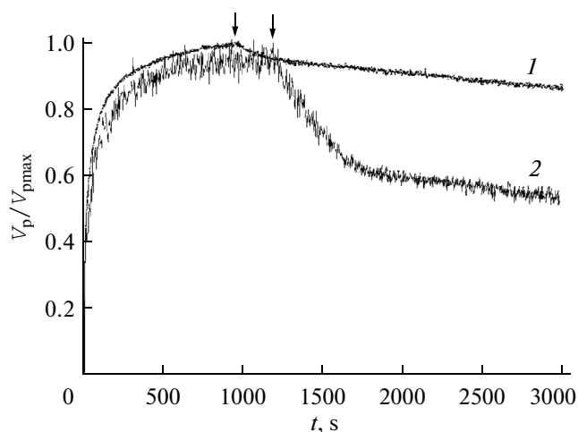
Fig. 3. Normalized plots of the dependence V_p(t) for the FPC samples based on PVA containing (1) 1 and (2) 10 wt % of dye RC. The moment of turning off light is marked with an arrow.
