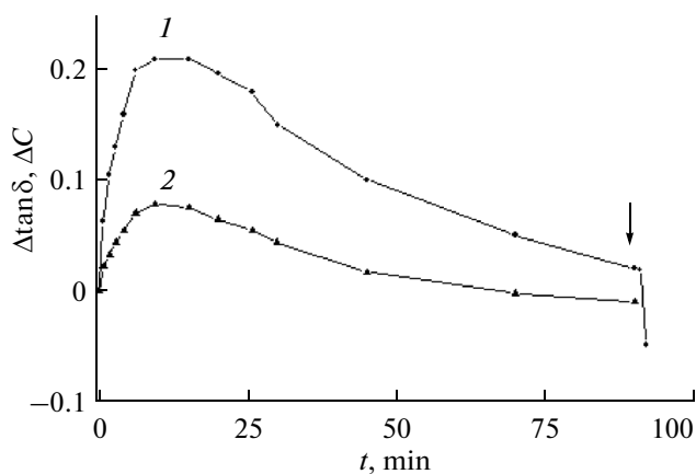
Fig. 5. Plots of time dependences of (1) \Delta \tan \delta and (2) \Delta C for the FPC samples based on PVA containing 10 wt % of dye RC. The moment of turning off light is marked with an arrow.
