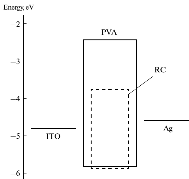
Fig. 2. Energy diagram of the FPC samples.
