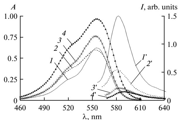
Fig. 1. (1–4) Absorption and (1'–4'') fluorescence spectra of FPCs based on PVA containing (1, 1') 1, (2, 2') 5, (3, 3') 10, and (4, 4') 20 wt % of dye RC.
