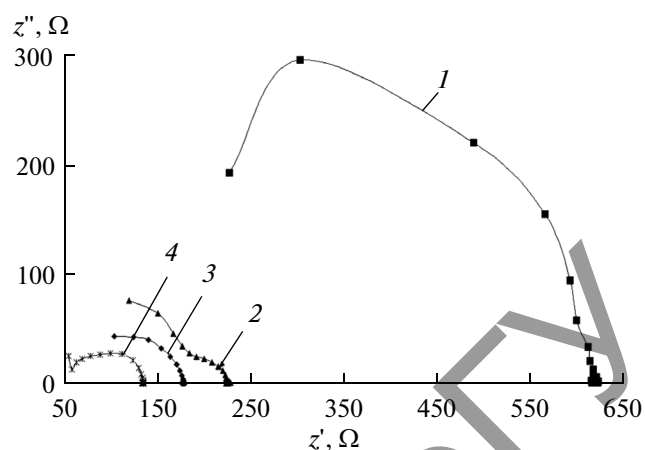
Fig. 4. Plots of electrical impedance spectra for the FPC samples (1) based on PVA and (2–4) containing dye RC: (2) 5, (3) 10, and (4) 20 wt % of dye RC.
