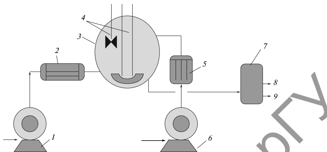
Process flow chart of the extraction of phenols from the tar of AO Sary-Arka Spetskoks: (1, 6) pumps, (2) heat exchanger, (3) extractor, (4) anchor and paddle stirrers, (5) vortex cavitation heater, (7) collector, (8) extract outlet, and (9) phenol-free tar outlet.
