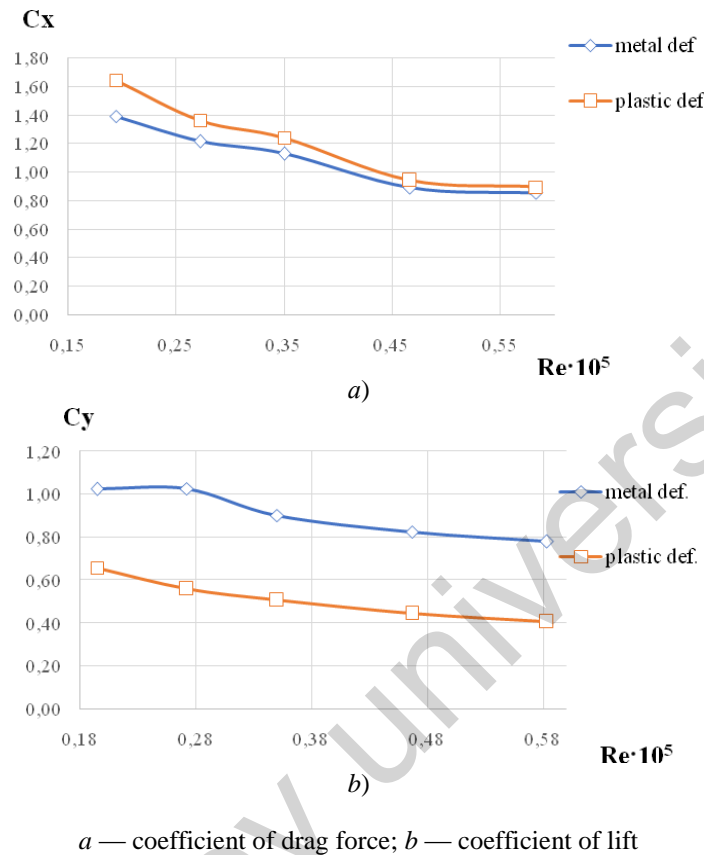
Figure 7. Dependence of aerodynamic coefficients on the Reynolds number
