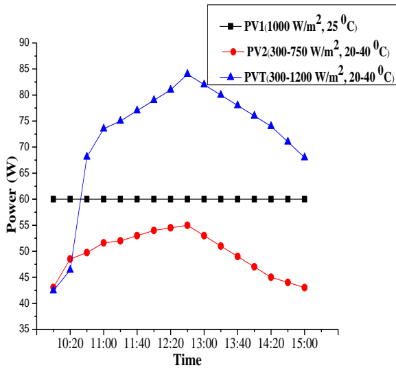
Fig. 7. Power values of 60 W PV based on PV/T with NTCS and 60 W PVB depending on time.
