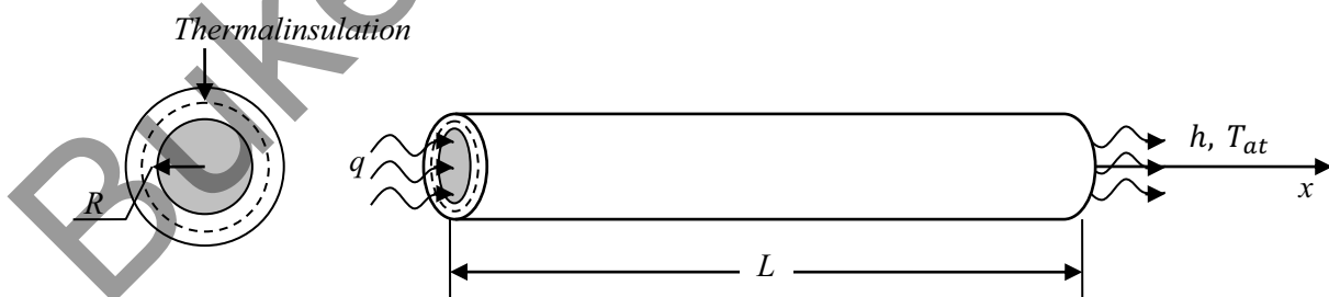
Figure1. Thermally insulated full rod
