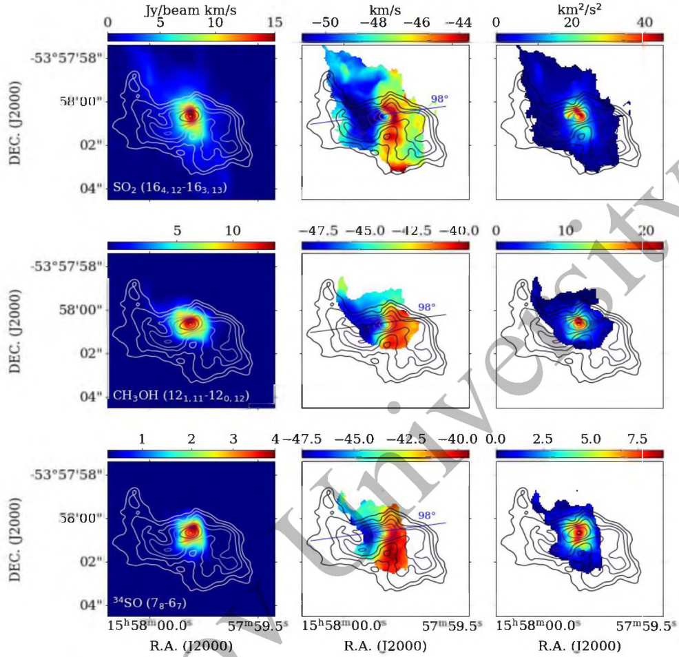
Fig.3. Moment 0, 1 and 2 maps of \text{SO}_2(16_{4,12}-16_{3,13}) , \text{CH}_3\text{OH}(12_{1,11}-12_{0,12}) and ^{34}\text{SO}(7_8-6_7) emission toward G328.2551–0.5321 A. Contour levels are 0.00267, 0.00405, 0.00615, 0.00934, 0.01418, 0.02152, 0.03267 and 0.04960 \text{Jy beam}^{-1} \text{ km s}^{-1} . The black ellipse in the lower-right panel denotes the synthesized beam.
