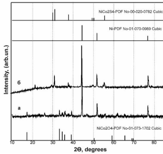
Figure 1. XRD pattern of synthesized samples \text{NiCo}_2\text{O}_4 (a) and \text{NiCo}_2\text{S}_4 (b)
