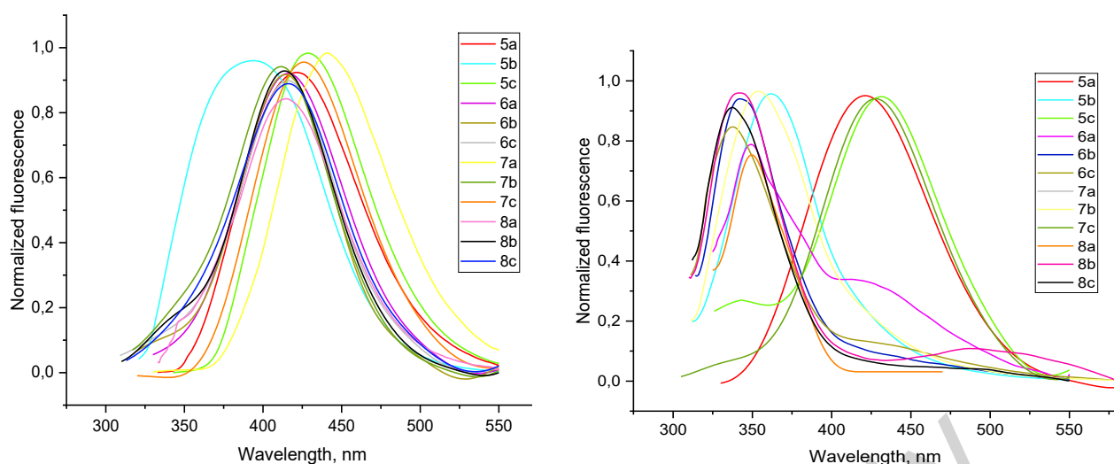
Figure 4. Normalized fluorescence spectra of oxazolo[5,4-b]pyridine derivatives 5-8a-c in acetonitrile (left) and toluene (right) solutions ( 6 \times 10^{-4} mol/L)
