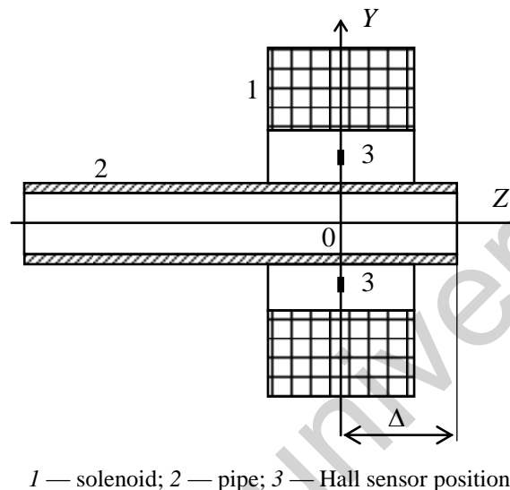
Figure 1. Ferromagnetic pipe in the magnetic field of the short solenoid
