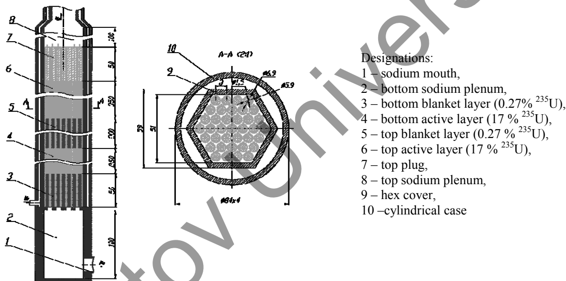
Fig.3. Design of the irradiation device.
