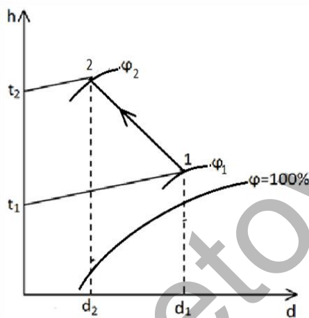
Fig. 3. The process of drying the working air when passing through the adsorption rotor.
