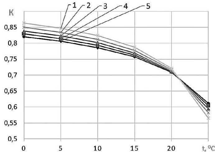
Fig. 5. Dependence of the recirculation coefficient on the fresh air temperature of the recuperator efficiency coefficient at a regeneration air temperature of 60 °C: 1- \eta_{rec} = 0.8 ; 2- \eta_{rec} = 0.6 ; 3- \eta_{rec} = 0.4 ; 4- \eta_{rec} = 0.2 ; 5- a system with a heat pump but without a recuperator.
