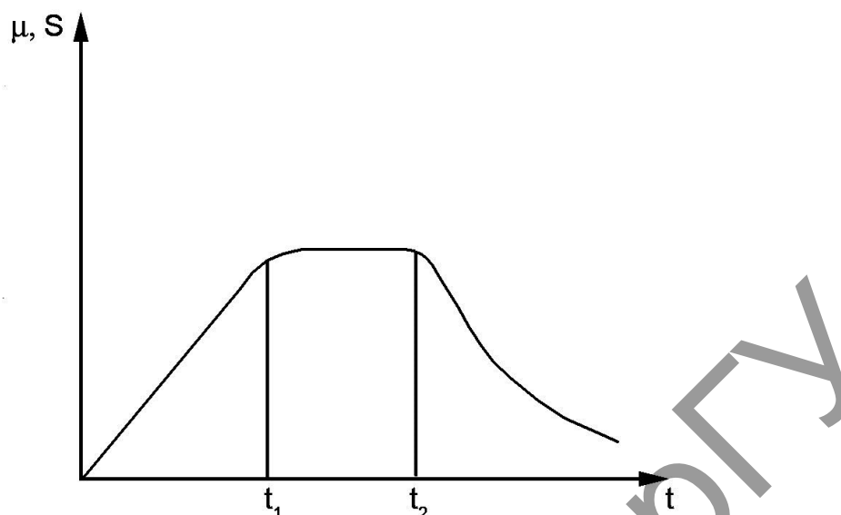
Figure 5. Three stages of temperature dependence of the optical absorption coefficient ( \mu ) of F-centers and stored energy ( S ) on temperature ( t C).
