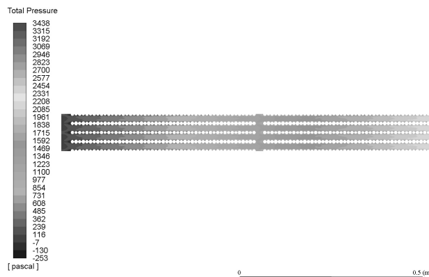
Figure 7. Pressure drop across a HE channel for a side ventilation system, Pa
