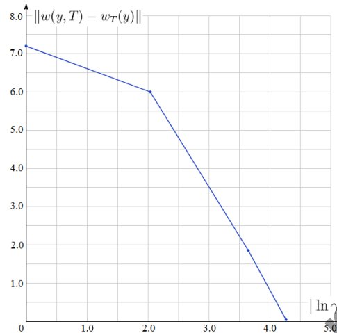
Fig. 5. Graph of the values of the minimized functional (excluding the regularizing term)
