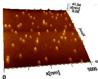
Figure 2. Microphotographs of scanning probe microscopy of PLGA-INH-NPs
