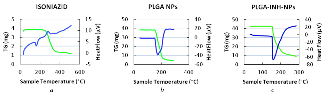
Figure 5. Thermogravimetric curves of INH (a), PLGA-NPs (b) and PLGA-INH-NPs (c)
