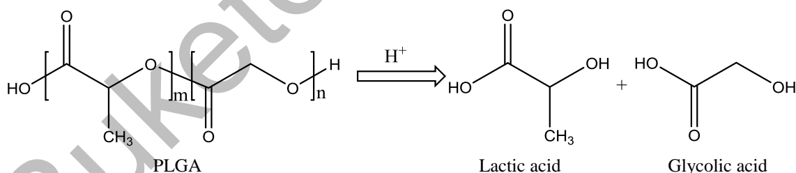
Figure 6. Degradation of poly(lactide-co-glycolide) to lactic and glycolic acid
