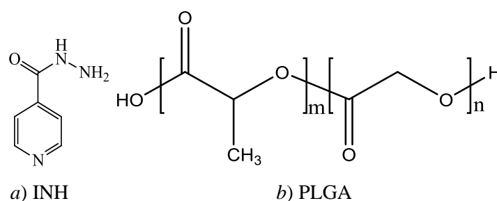
Figure 1. Structural formula of isoniazid and poly(lactide-co-glycolide)
