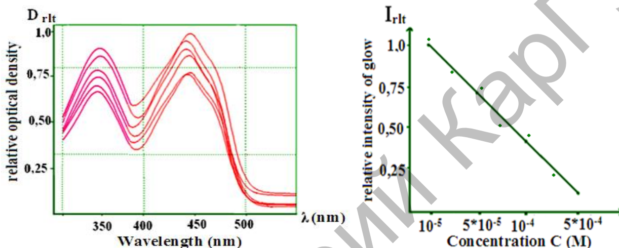
Fig.1a. Absorption spectrum of riboflavin ( C 10^{-4} \text{ M} ) in a binary mixture of alcohol + acetone solvents depending on the fraction of acetone added (0-1, 20-2, 30-3, 50-4, 70-5) in% by volume ratio.
