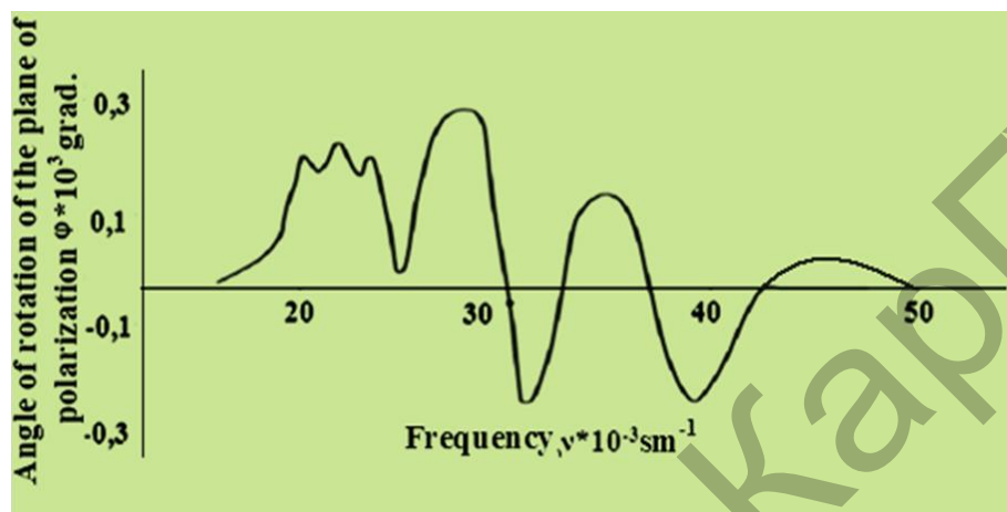
Fig.3. The spectrum of linear dichroism of self-assembled riboflavin molecules in a laminar hydrodynamic flow
