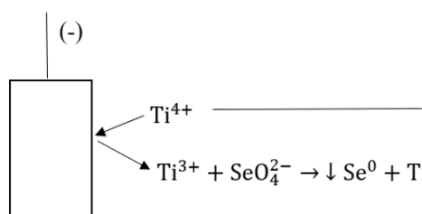
Scheme 1. Scheme for the reduction of hard-to-reduce selenium (VI) anions at the cathode in the presence of variable-valent cations
