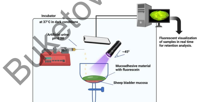
Figure 1. Experimental setup for investigating the retention of mucoadhesive formulations on the bladder mucosa
