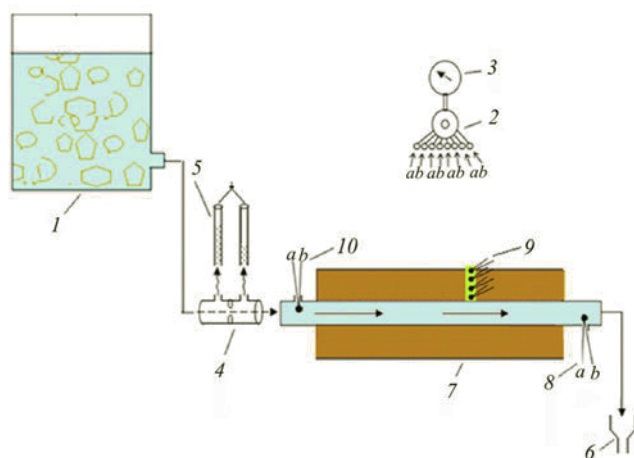
Fig. 1. Experimental bench for modeling of heat-transfer processes in heat-removal elements of a heat pump for "ground–water" systems: 1) thermostat; 2) switch of thermocouples; 3) potentiometer to measure the thermocouples' emf; 4) orifice plate of the heat-removal portion; 5) differential manometer; 6) outlet pipe of the municipal sewer; 7) heat-transfer portion with sand; 8, 9, and 10) thermocouples (a and b are thermocouple connectors).
