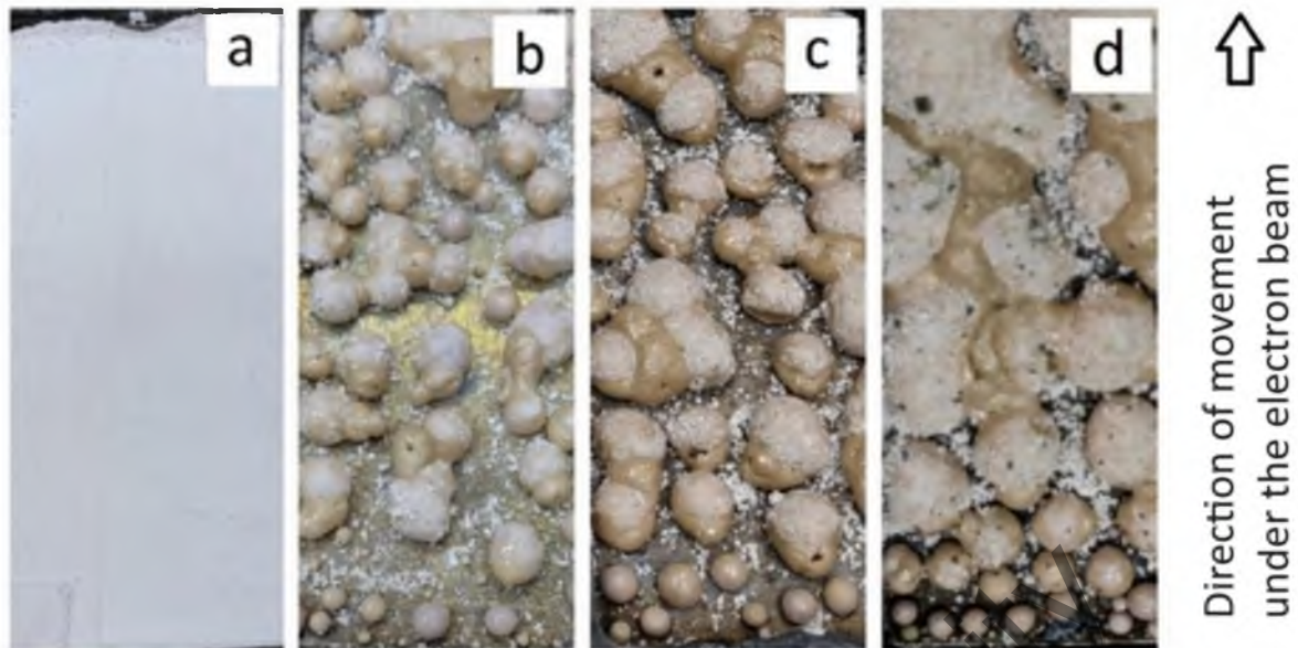
Figure 1. Effect of beam energy on melting results:
