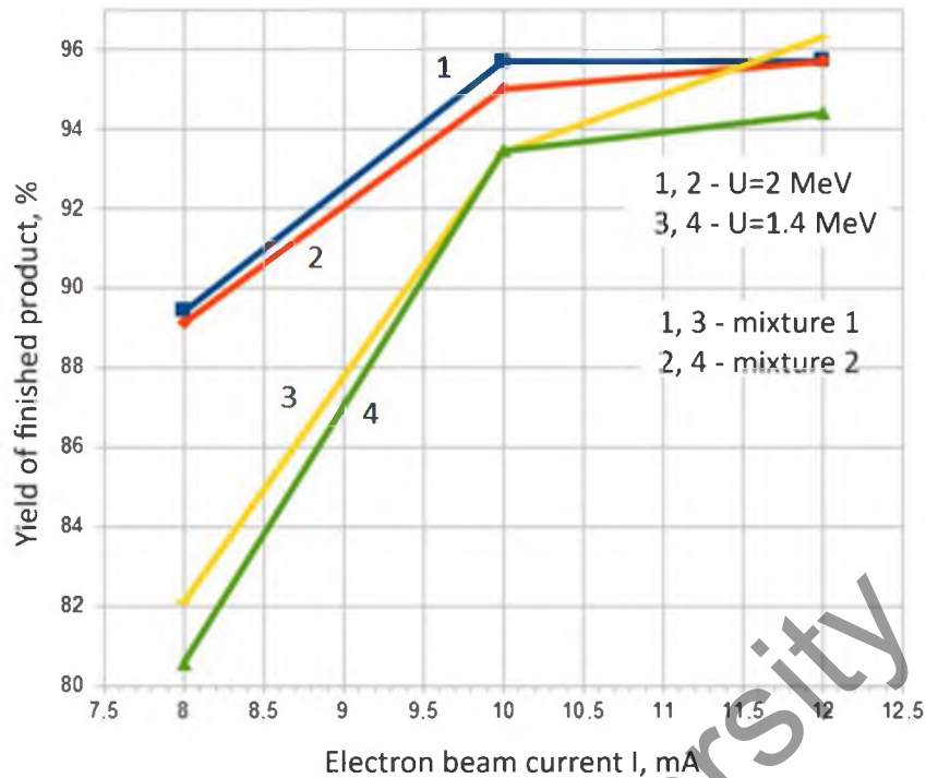
Figure 5. Dependences of the melting efficiency of mixture 1 and mixture 2 at an accelerating beam voltage of 1.4 MeV and 2 MeV on the beam current
