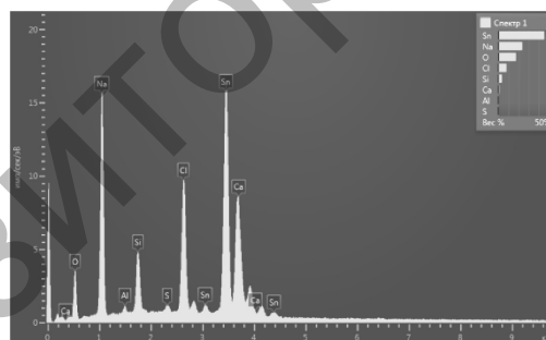
Figure 4. Element structure of a film with aluminium oxide (zone «spectrum 1»)
