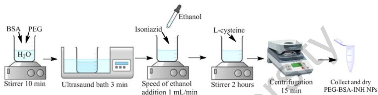
Figure 2. Scheme for producing PEG-BSA-INH nanoparticles
