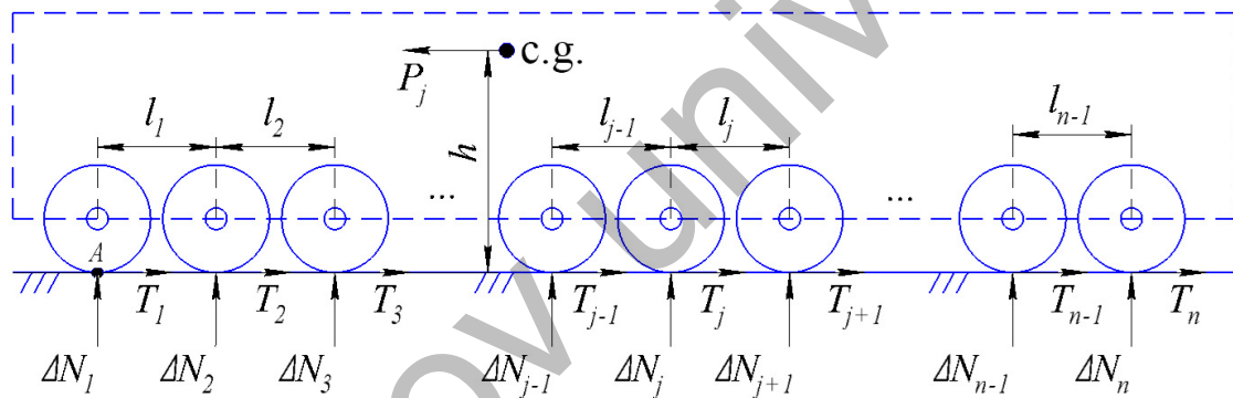
( T_1, T_2, T_3, T_{j-1}, T_j, T_{j+1}, T_{n-1}, T_n are braking forces on the corresponding axles of the n -axle WV; l_1, l_2, l_{j-1}, l_j, l_{n-1} are the distances between the corresponding axles of the n -axle WV; h is the height of the center of gravity (c.g.) of the WV; P_j is the inertia force of the braking n -axle WV).
