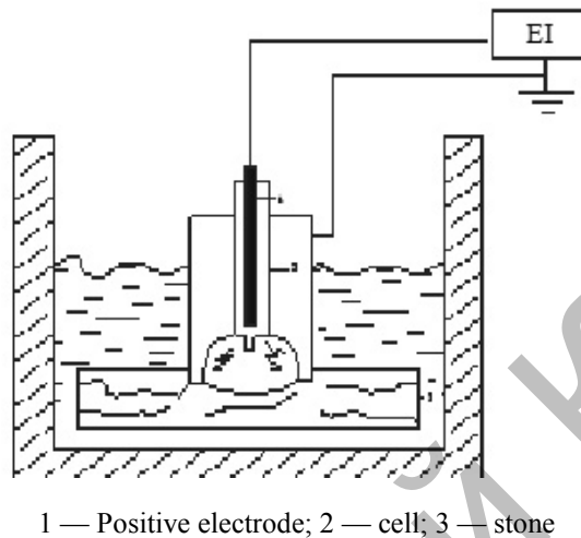
Figure 3. Scheme of the electro-hydraulic drilling
