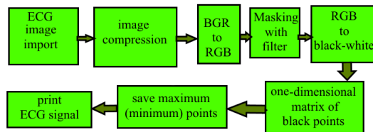
Fig. 3. Block diagram of the proposed algorithm of image processing.
