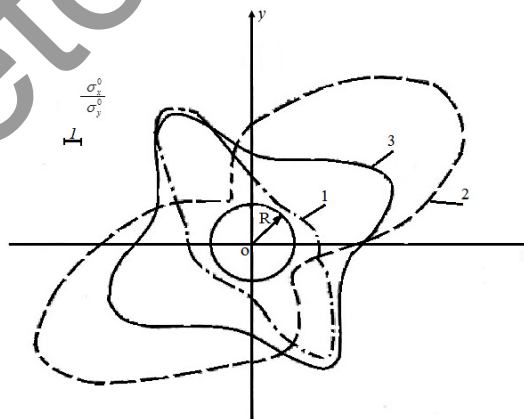
Fig.4. Plots of normal stresses on the contour of a field preparatory drift.
