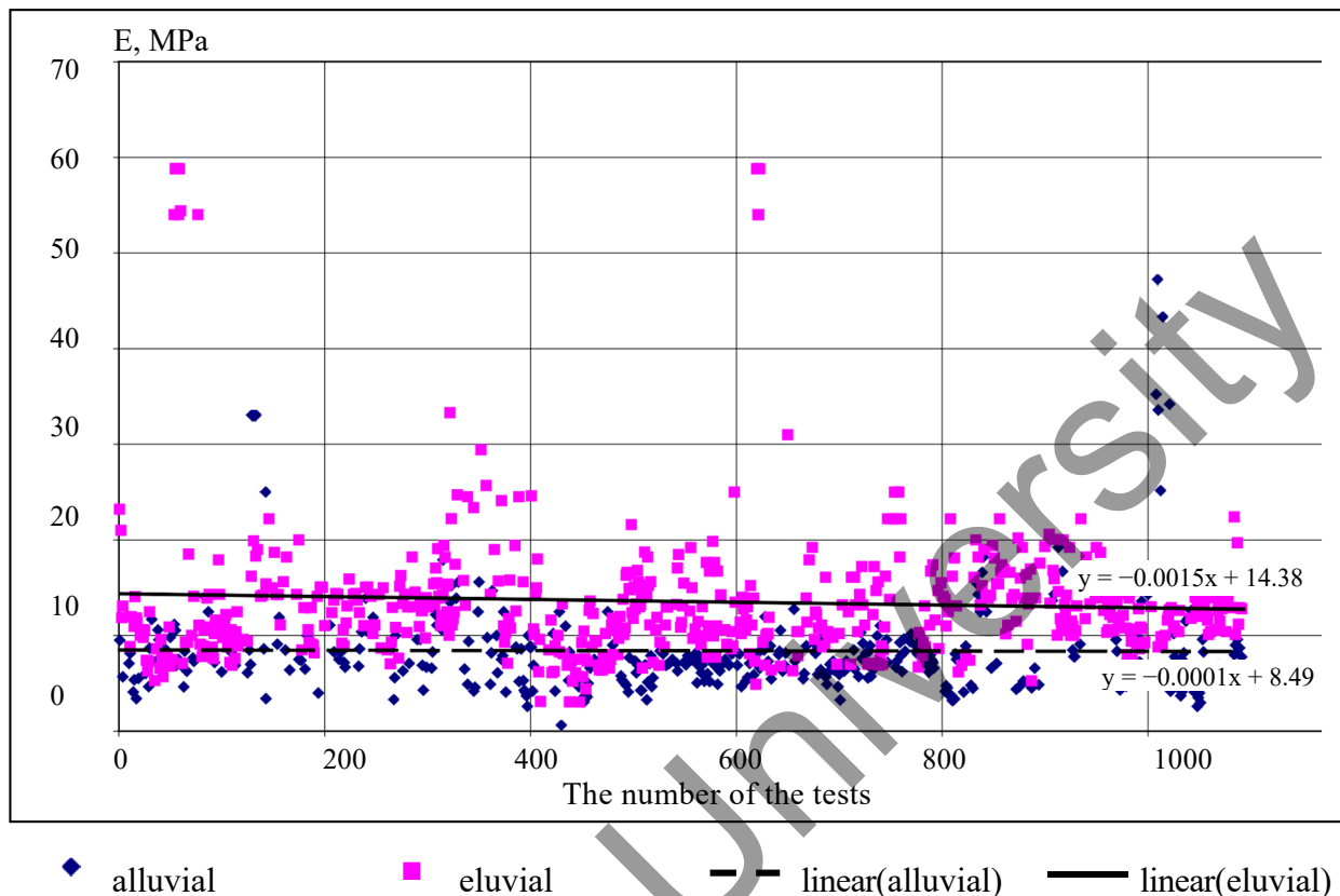
Figure 6. Deformation modulus E scatter plot for alluvial and eluvial clay deposits.
