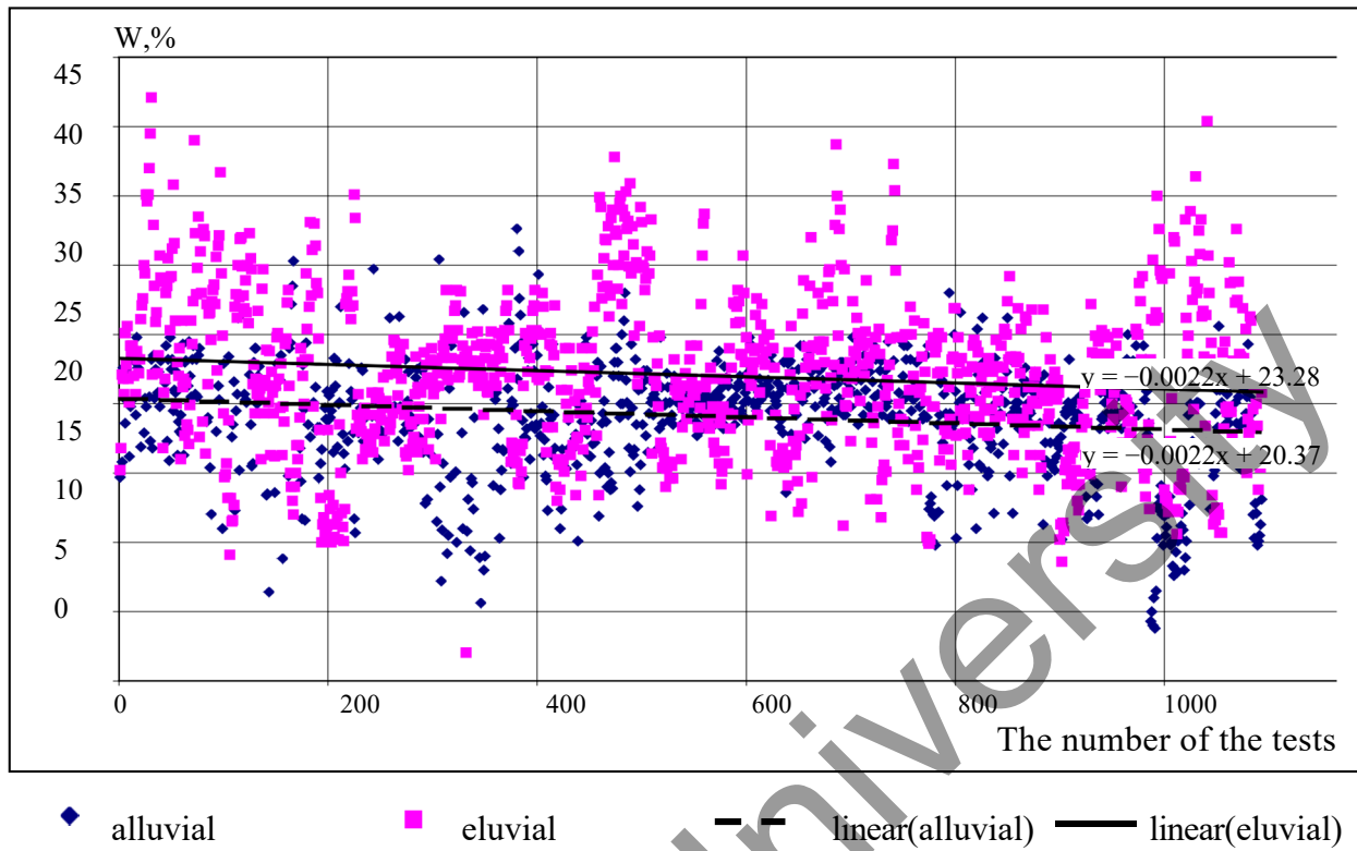
Figure 4. Scatter plot of the natural moisture content for alluvial and eluvial clay soils.
