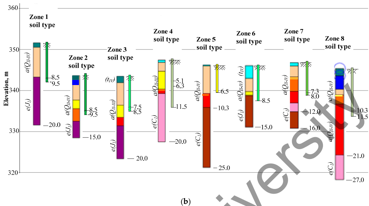
Figure 8. Zoning map for optimization of pile lengths (a) and representative borehole profiles (b) for each city zone.
