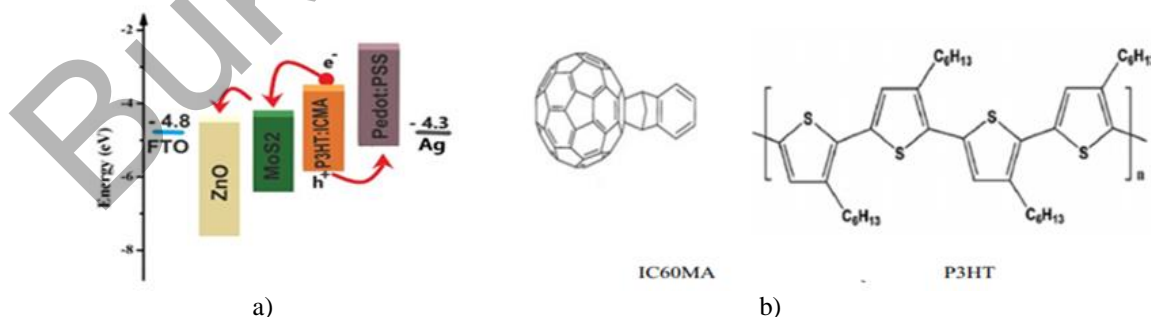
Fig.5 (a) Energy level diagram of ZnO:MoS 2 and (b) chemical structures of BHJ compounds
