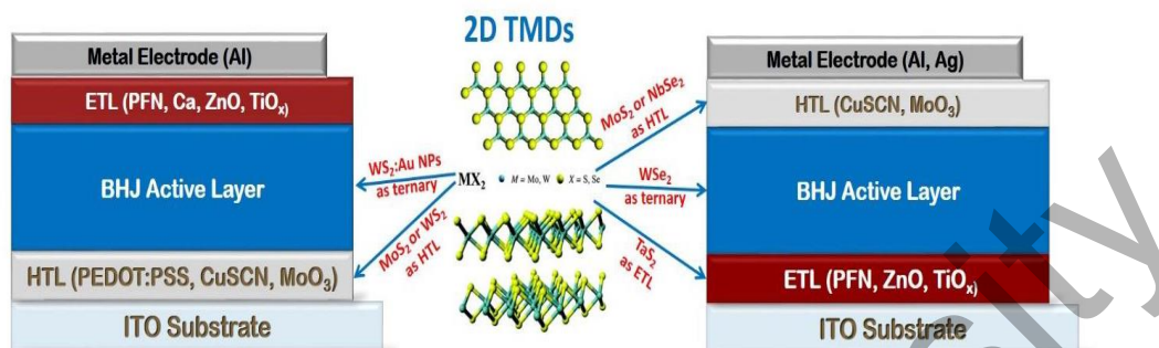
Fig. 1. Schematic diagram showing both the direct (left) and inverted OPVs structure. In the center the structure of various 2D TMDs are shown, and the blue arrows show the various layers in which TMDs were added [1].
