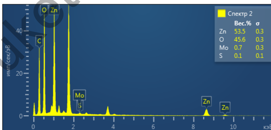
Fig.3. EDX analysis
