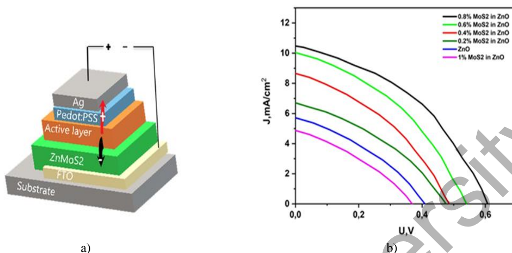
Fig.6. a) the architecture of the inverted PSC b) J–V characteristics of inverted solar cells
