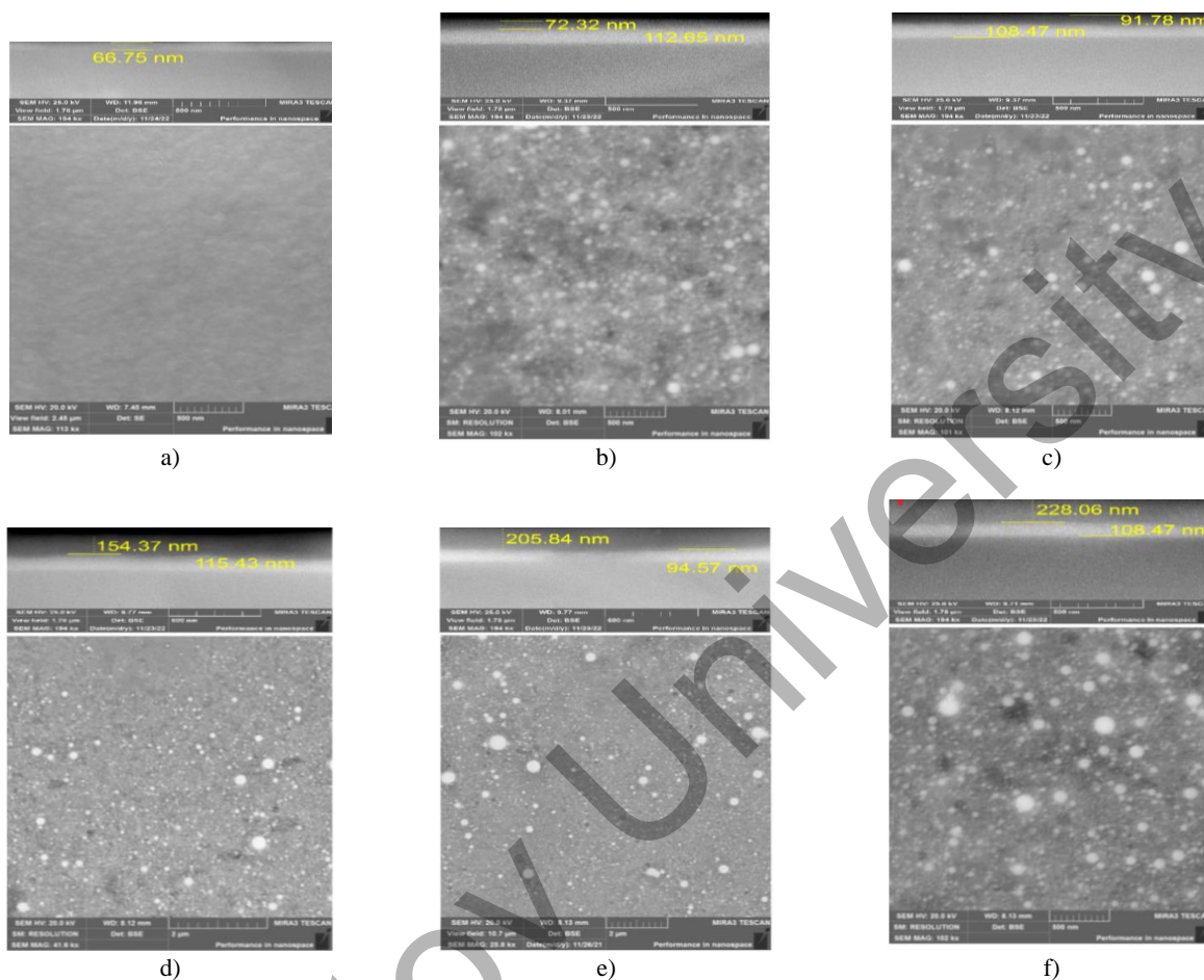
Fig. 2. Images of surface morphology of ZnO:MoS 2 composite films
