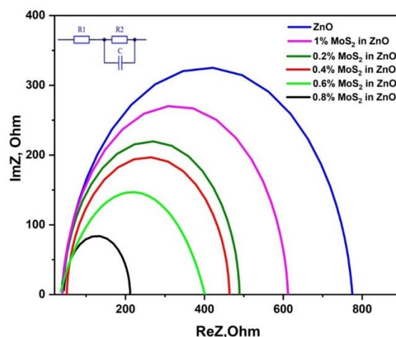
Fig.7. Impedance spectra of PSCs
