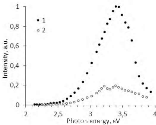
Figure 1. CL spectrum of Ga_2O_3 sample: 1 — taken at amplitude value of a pulse, 2 — in 200 ns.
