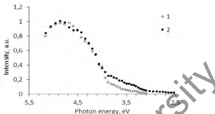
Figure 4. CL spectra of Al_2O_3 (1) and Al_2O_3 : Ce 0.5 % (2) samples.
