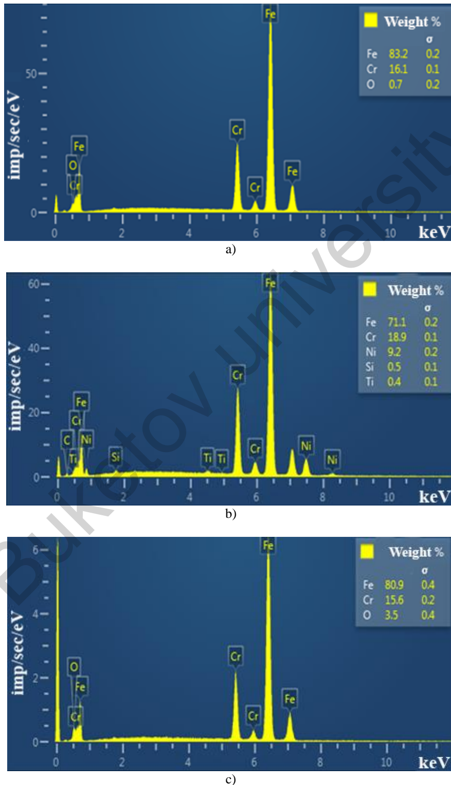
Fig.4. Energy-dispersive X-ray spectra: a) Percentage content of elements in untreated X17 stainless steel; b) Percentage content of elements in X19N9T stainless steel; c) Component composition of X17 steel after complex 6- hours treatment with air heated to 350 °C and UVT.
