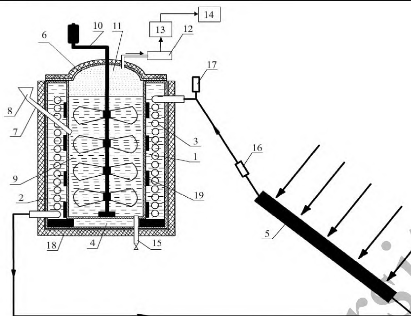
Fig. 1. Schematic diagram of a solar biogas plant. (FAP 2440 19.03.2024): 1 - reactor of biogas device; 2 - water reservoir; 3 - helical heat exchanger made of plastic tube; 4 - water in Reservoir jacket; 5-solar water heater collectors; 6 - reservoir and reactor top seal; 7 and 8 - reactor ready biomass injector Hatch and its throat; 9-biomass in reactor; 10 - mixer device; 11 - formed biogas; 12 - throttle; 13 - gas filter 14 - gas kraynik; 15 - humus release lug; 16 - thermoregulator; 17 - expansion tank; 18 - external thermal insulation; 19 - phase variable heat-collecting material
