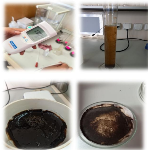
Fig. 6: Acidification and precipitation of humic acids.
