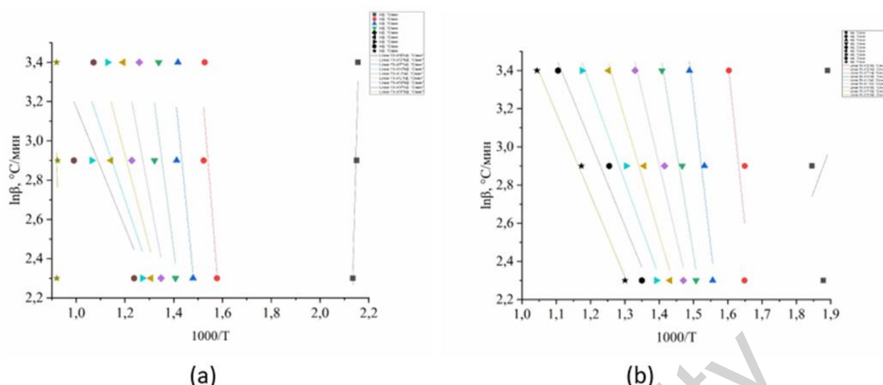
Fig. 5: Dependence of the logarithm of the heating rate on the return temperature.
