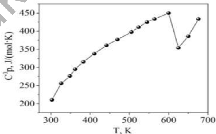
Figure. Diagram of dependence of heat capacity on temperature LaCaTiMnO 6
