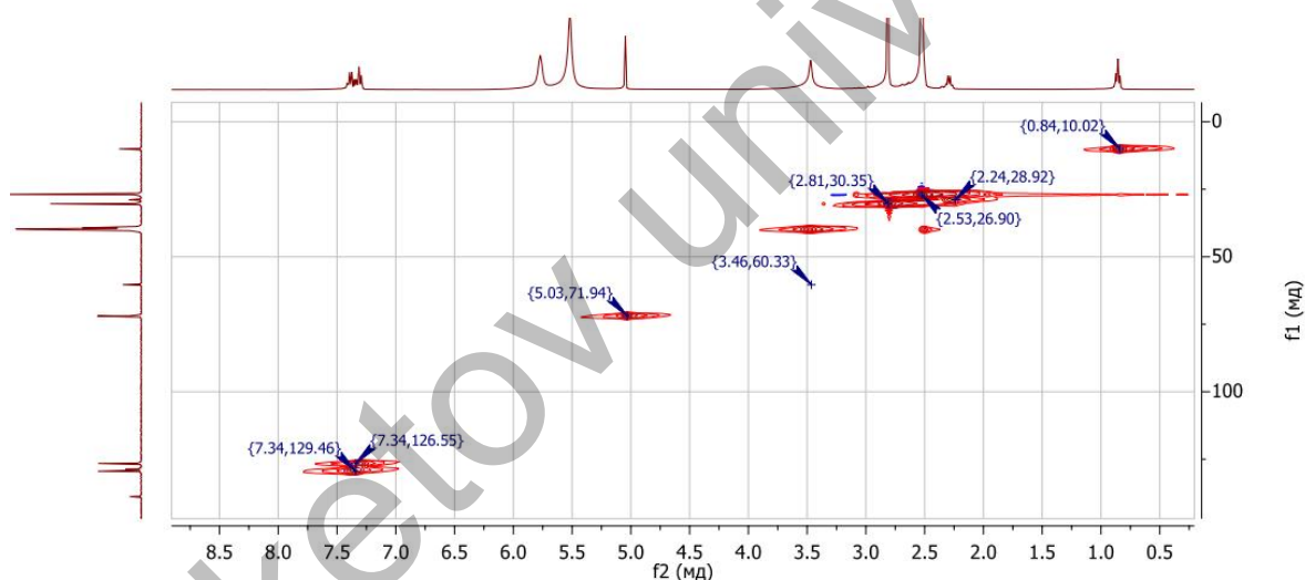
Figure 5. ^1\text{H} - ^{13}\text{C} HSQC spectrum of a model mixture of substances: urea I , barbituric acid II , phenobarbital IV , N,N'-dimethylurea XIX and N-methylglycoluril X in DMSO- d_6 ( \delta : 2.50 ppm; 39.5 ppm)
