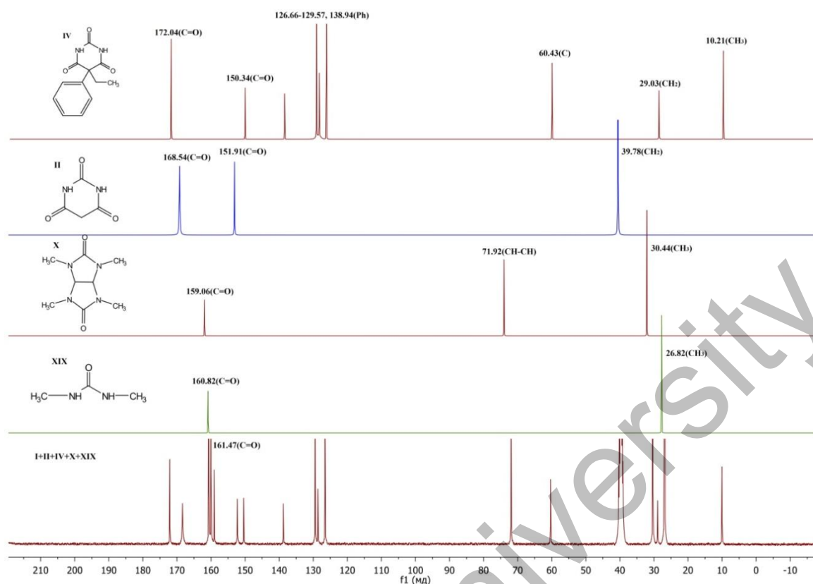
Figure 3. ^{13}\text{C} NMR spectrum of a model mixture of substances: urea I , barbituric acid II , phenobarbital IV , N,N'-dimethylurea XIX and N-methylglycoluril X in \text{DMSO-d}_6 ( \delta 39.5 ppm)
