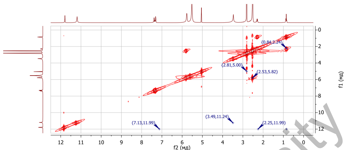
Figure 4. ^1\text{H} - ^1\text{H} COSY spectrum of a model mixture of substances: urea I , barbituric acid II , phenobarbital IV , N,N'-dimethylurea XIX and N-methylglycoluril X in DMSO- d_6 ( \delta : 2.50 ppm)
