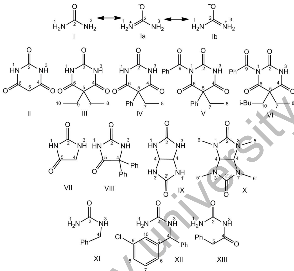
Figure 1. Structures of substances I–XIII
