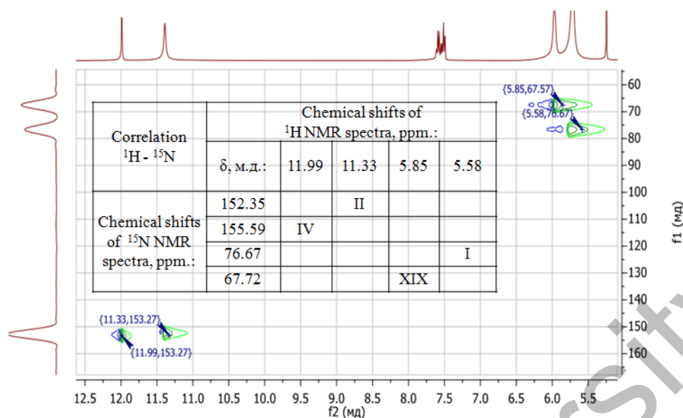
Figure 6. ^1\text{H}-^{15}\text{N} HSQC spectrum of a model mixture of substances: urea I , barbituric acid II , phenobarbital IV , N,N'-dimethylurea XIX and N-methylglycoluril X in DMSO- d_6 ( \delta 2,50 ppm)
