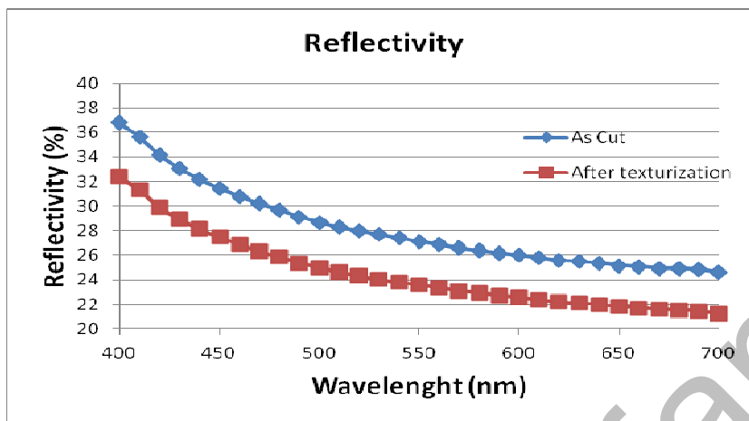
Figure 2. The reflectivity before and after texturing, obtained by spherical spectrometry on X-Rite SP62 reflectometer
