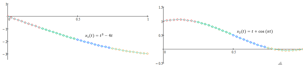
Figure 1. The exact solution values are indicated by the light blue solid line and the numerical solution values obtained by the Bulirsch-Stoer method are indicated by the symbol \circ
