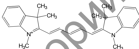
Figure 1. Structure of cyanine dye
