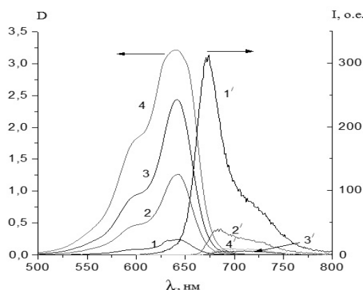
Figure 2. The concentration dependence of the absorption (1–4) and fluorescence (1'–4') ( \lambda_{ex}=590 nm) spectra of dye at various concentrations
