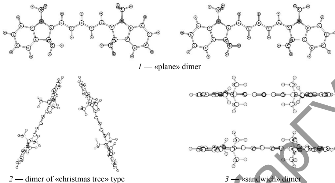
Figure 7. The calculated conformation of dye dimers
