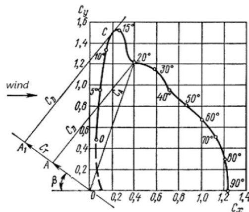
Figure 3. Polar of the sail
