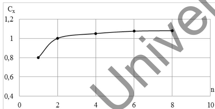
Figure 10. Dependence of the aerodynamic coefficient (drag) on n
