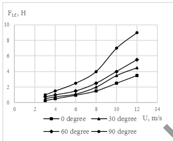
Figure 4. Graph of dependences of the lift forcing of the sail blade on the flow velocity at various angles \gamma of the apex of the triangular blade
