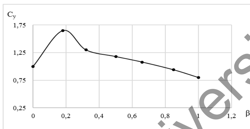
Figure 7. Dependence of the aerodynamic coefficient (lift) from \beta
