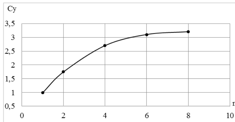
Figure 9. Dependence of the aerodynamic coefficient (lift) from n
