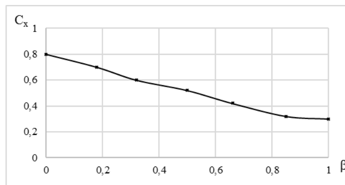
Figure 6. Dependence of the aerodynamic coefficient (drag) from \beta
