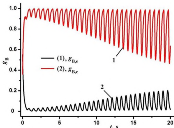
Fig. 3. Changes in the concentration of g_{B,c} and g_{B,e} for 20 s after "launch".
