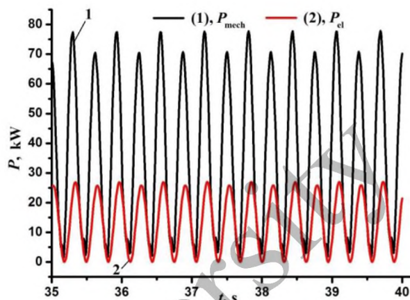
Fig. 4. Changes in powers P_{\text{el}} and P_{\text{mech}} during averaging time from 35 to 40 s.
