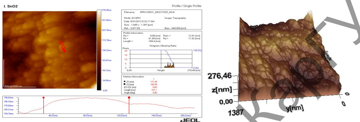
Figure 4. AFM images of a surface of a porous tin oxide obtained at room temperature in \text{NH}_4\text{OH} .
