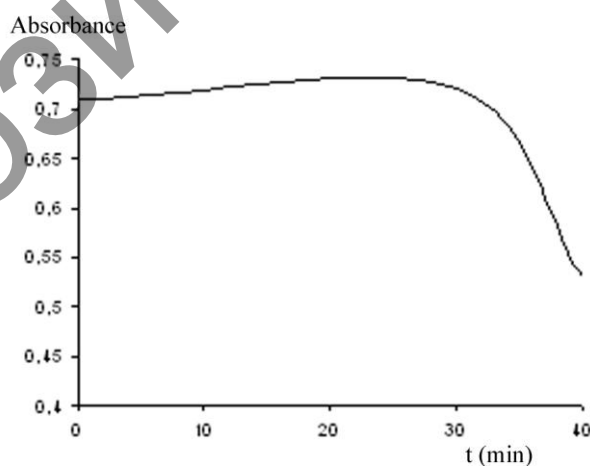
Figure 7. The dependence of the optical density of D149 dye versus sorption time into anodized Sn.
