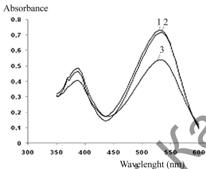
Figure 6. The absorption spectra of the D149 dye before and after sorption: 1 – before sorption 2 - 30 min sorption 3 - 40 min.
