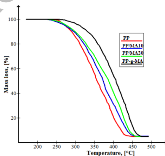
Figure 8. TGA of PP and PP-g-MA blends
