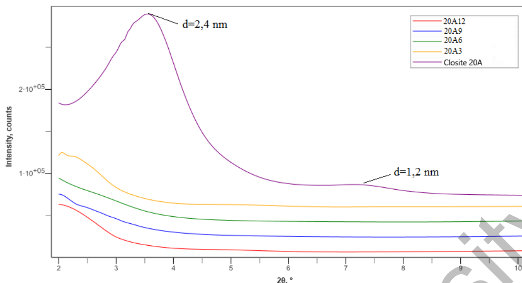
Figure 2. PP and Cloisite20A composites small angle X-ray curves.
