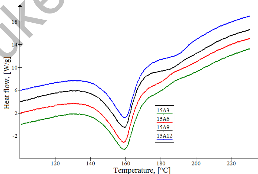
Figure 6. DSC curves of composites with Cloisite15A
