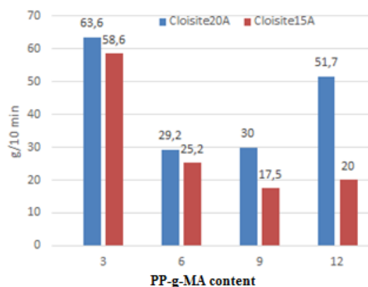
Figure 4. MFI of composites based on Cloisite15A and Cloisite20A
