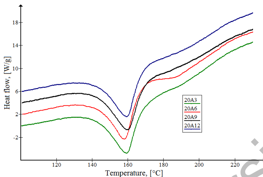
Figure 7. DSC curves of composites with Cloisite20A
