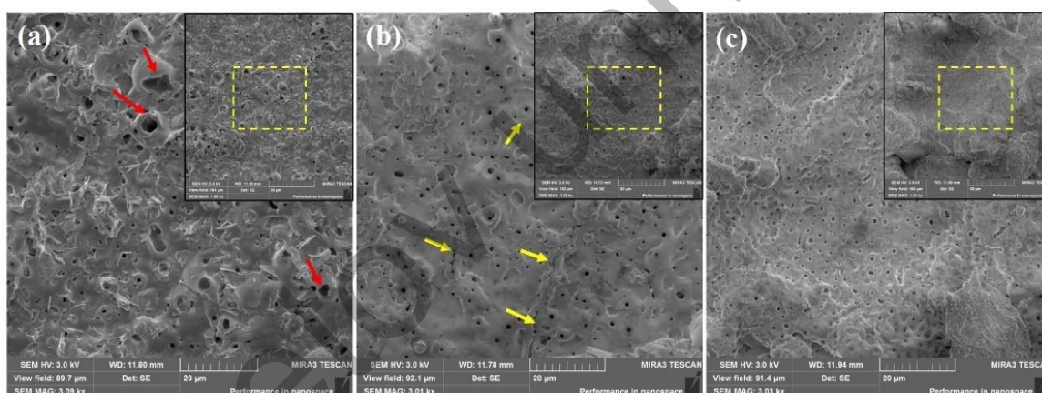
Figure 2. Surface morphology of PEO coatings of various electrolytes (a) H, (b) P, (c) S
