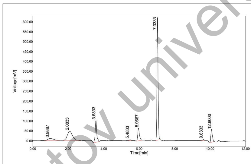
Figure 7: UV light degradation chromatogram of darolutamide
