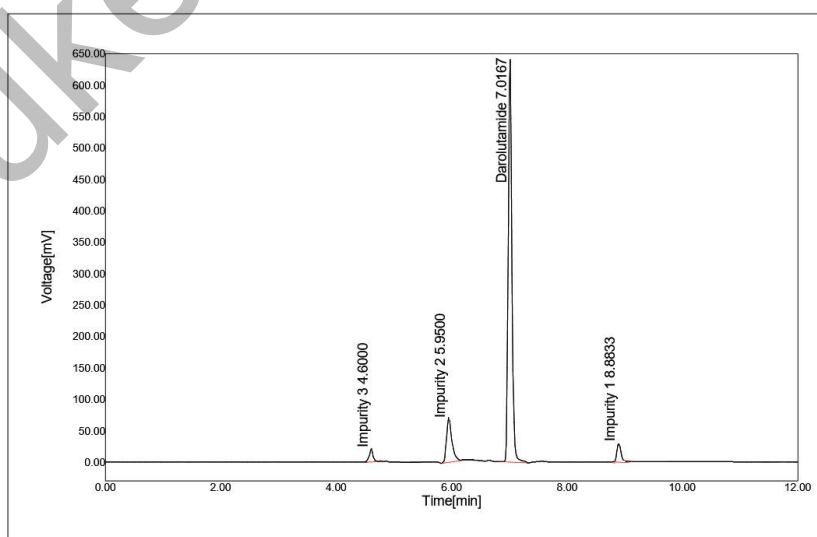
Figure 8: Formulation chromatogram of darolutamide
