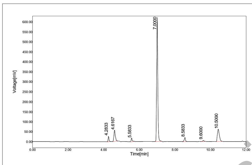
Figure 6: Thermal degradation chromatogram of darolutamide
