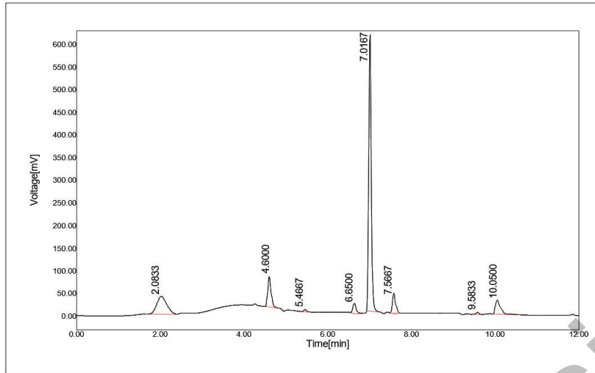
Figure 3. Acid degradation chromatogram of darolutamide
