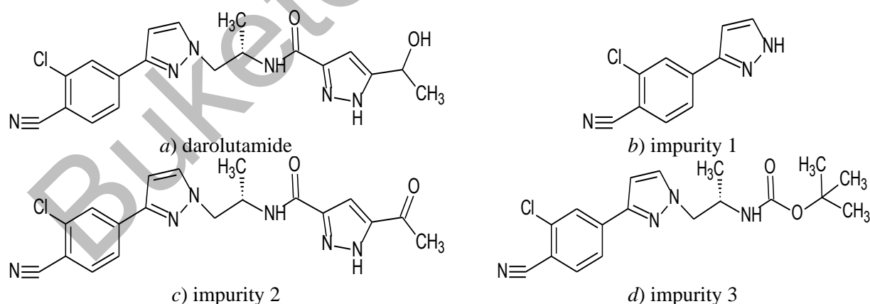
Figure 1. Chemical structure of darolutamide and its impurities in the study
