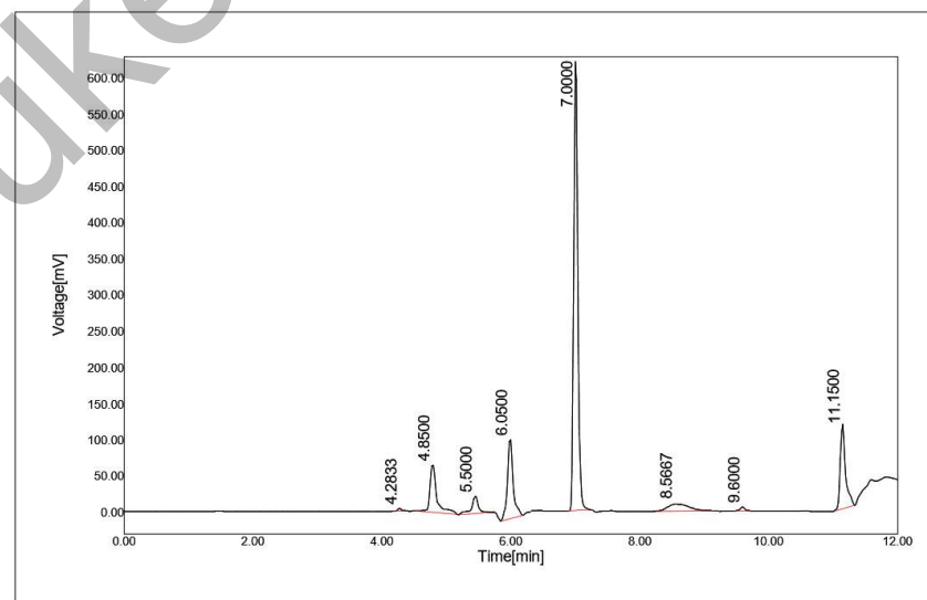
Figure 5. Peroxide degradation chromatogram of darolutamide
