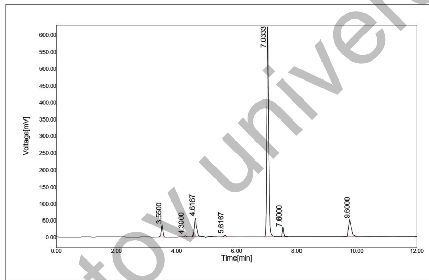
Figure 4. Base degradation chromatogram of darolutamide
