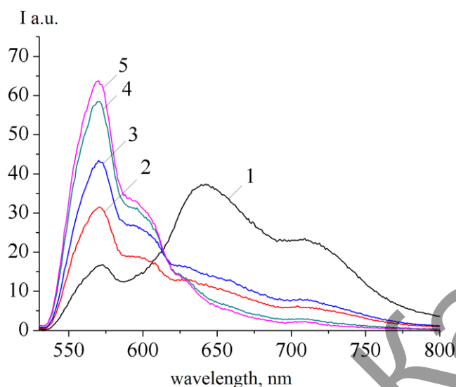
Fig.4. Fluorescence spectra of the films P3HT on the surface of the islet silver films obtained at different annealing temperatures: 1 – without NPs; 2 – 20 °C; 3 – 120 °C; 4 – 180 °C; 5 – 240 °C.
