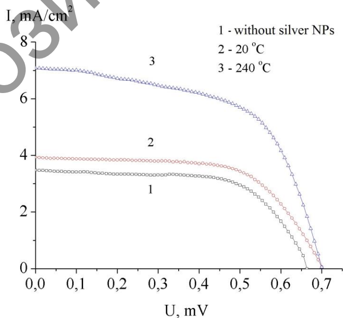
Fig.7. Current-voltage characteristics of organic solar cells with the islet silver films
