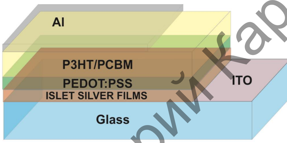
Fig.6. Design of organic solar cell with bulk heterojunction
