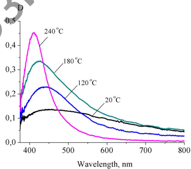
Fig.2. The plasmon absorption spectra of silver films prepared by spraying of metals in vacuum and subsequent annealing
