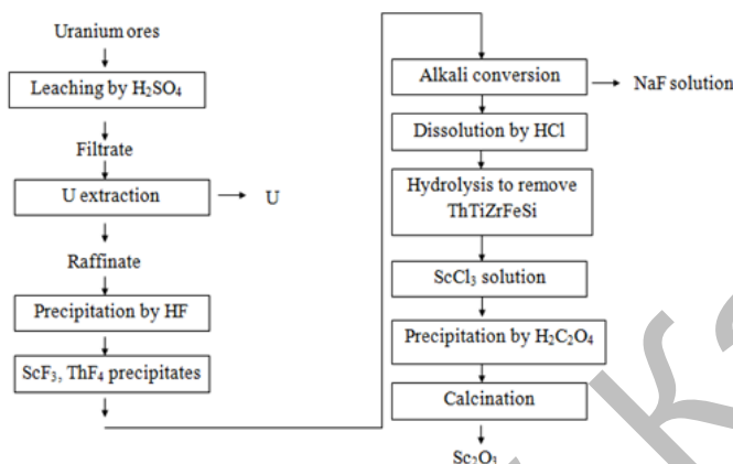
Figure 4. Scheme of scandium extraction from uranium ores
