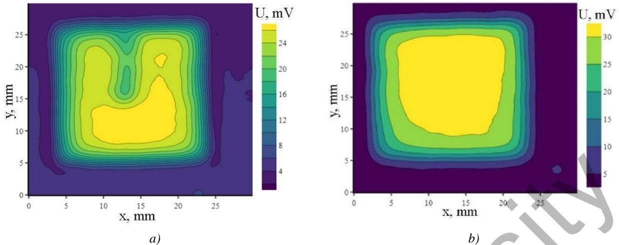
Fig. 5. Batch 1 scan results
