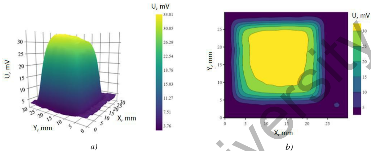
Fig. 4. Graphical representation of the result of scanning the research object in three-dimensional (a) and two-dimensional (b) form
