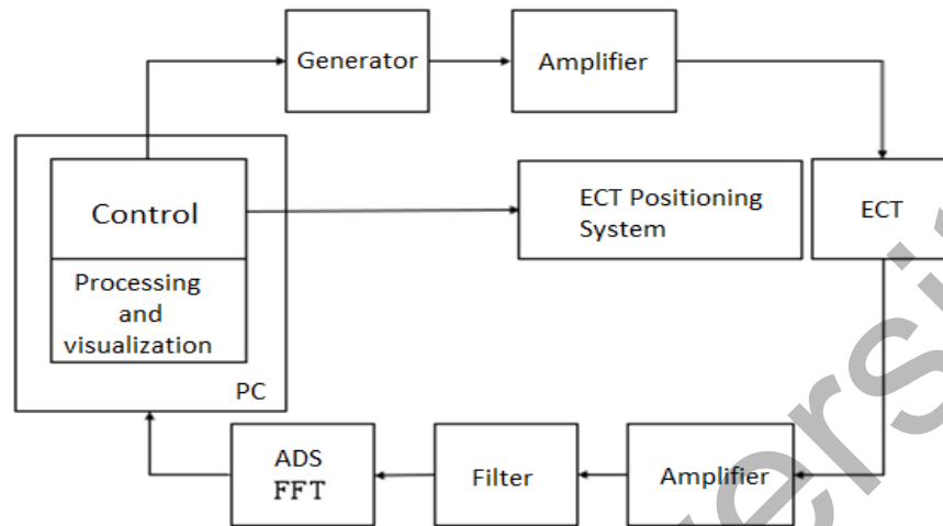
Fig.2. Scheme of the eddy current complex
