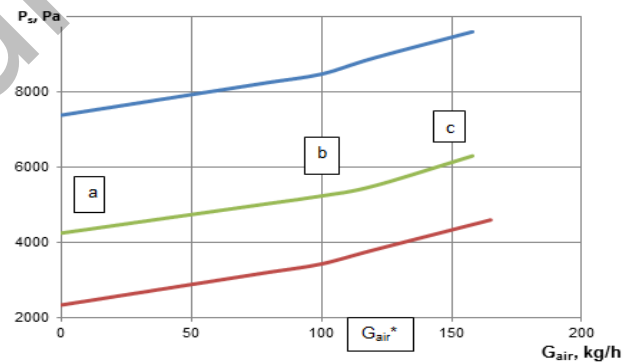
Fig.2. Curve of the 1st ejector stage EPO-2-80 for ejector sucking off the vapor-air mixture
