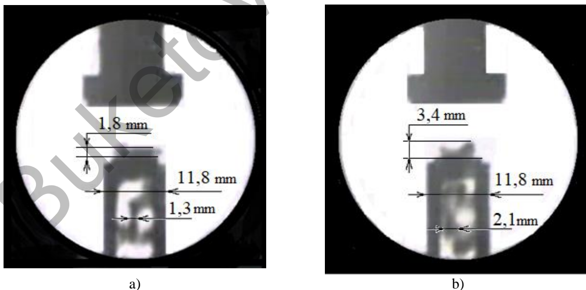
Figure 4. Shadow images of gas mixture separation zone in the upper chamber of diffusion cell for system 0.5143 He + 0.4857 Ar — N 2 at p = 2.54 MPa, T = 298.0 K: a) Initial stage of the process; b) Mode of periodic formation of vortex structures
