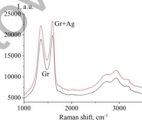
Figure 3. Raman spectra of Gr films deposited by airbrushing with the addition of Ag NPs
