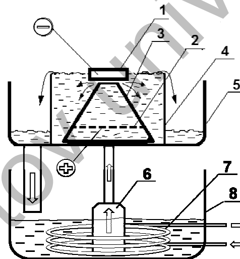
Fig.1. Scheme of the installation for electrolytic plasma treatment:
